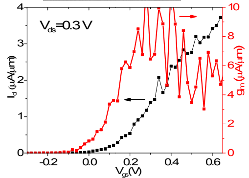
Fig. 6 Transfer characteristics at V_{ds}=0.3\text{ V} of the device shown in Fig. 5.
