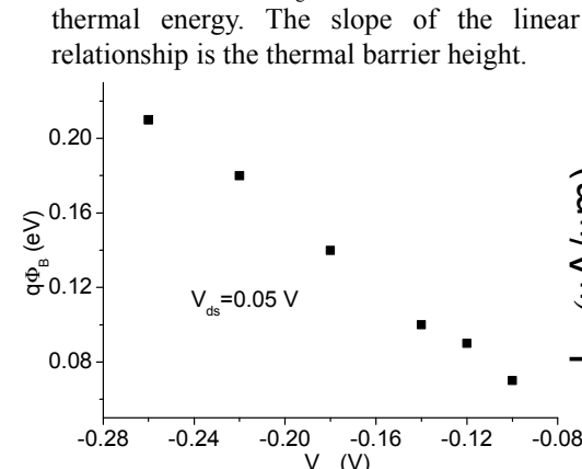
Fig. 15 Thermal barrier height extracted from the slopes in Fig. 14 as a function of V_{gs} .
