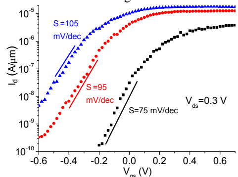
Fig. 9 Subthreshold characteristics of three single-NW TFETs at V_{ds}=0.3\text{ V} indicating device-to-device variability.
