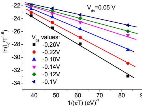
Fig. 14 Arrhenius plot of the subthreshold current at various V_{gs} values versus inverse thermal energy. The slope of the linear relationship is the thermal barrier height.
