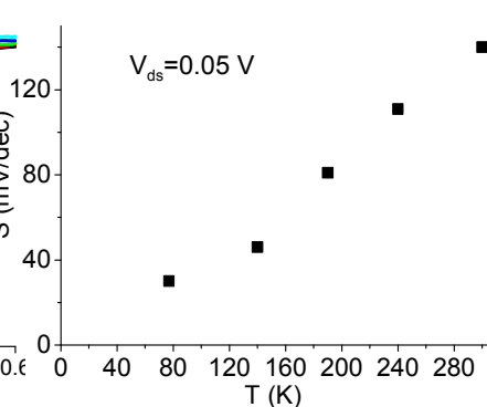
Fig. 13 Temperature dependence of the subthreshold slope S shown in Figs. 11 and 12.
