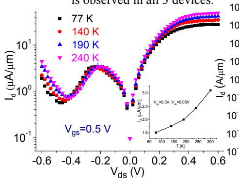
Fig. 11 I_d - V_{ds} characteristics at V_{gs}=0.5 V of a single-NW TFET in semilog scale at different temperatures from 77 to 240 K. Inset: I_d vs. T at V_{ds}=0.05 V, V_{gs}=0.5 V.
