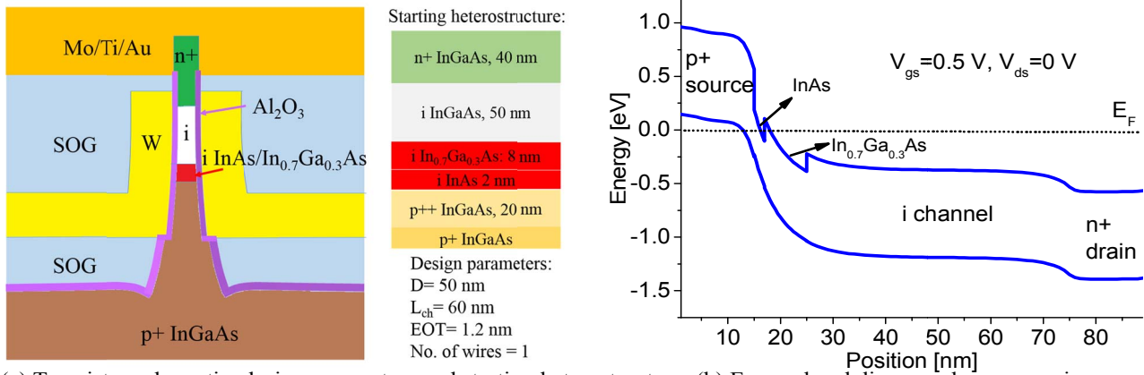
Fig. 1 (a) Transistor schematic, design parameters and starting heterostructure. (b) Energy band diagram along nanowire.
