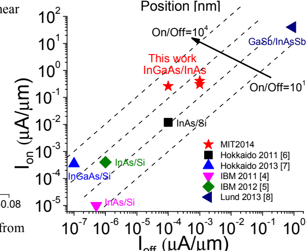
Fig. 17 I_{on} vs. I_{off} at V_{dd}=0.3 V ( V_{ds}=0.3 V, \Delta V_{gs}=0.3 V) for recently published vertical NW TFETs containing III-V materials. All devices but the present ones are fabricated through bottom-up techniques.
